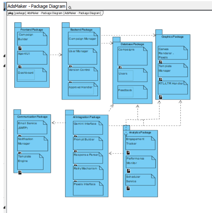
Figure 2 Package Diagram
