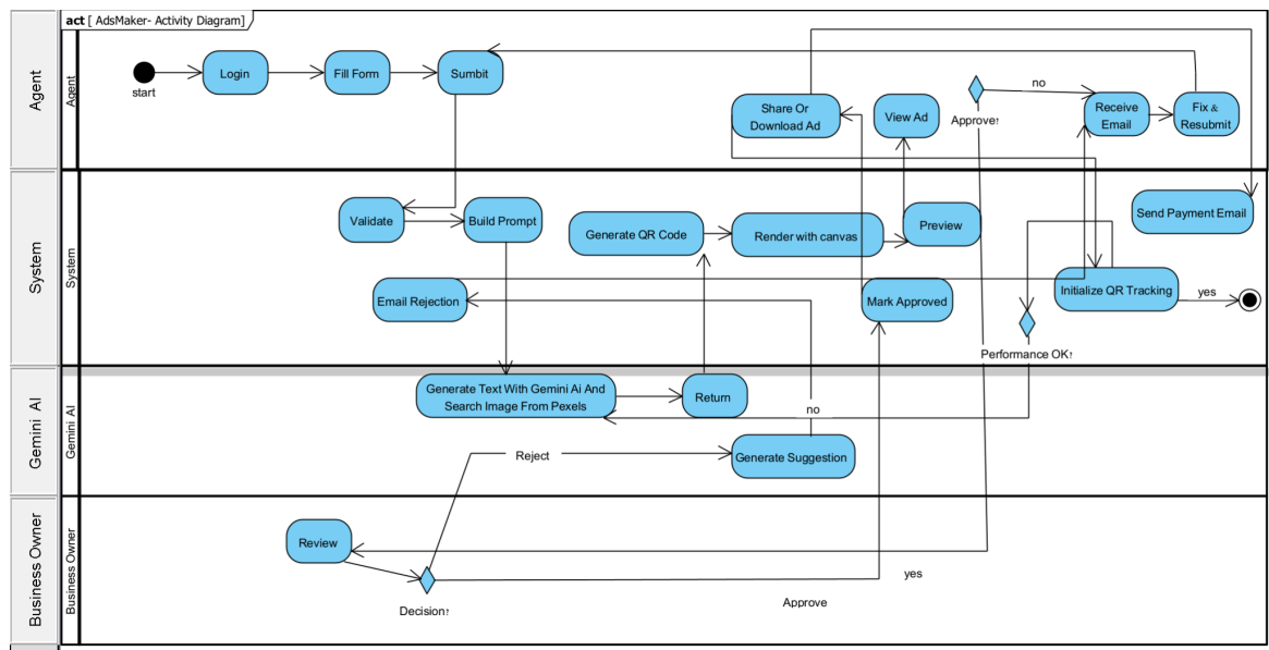
Figure 3 Activity diagram
